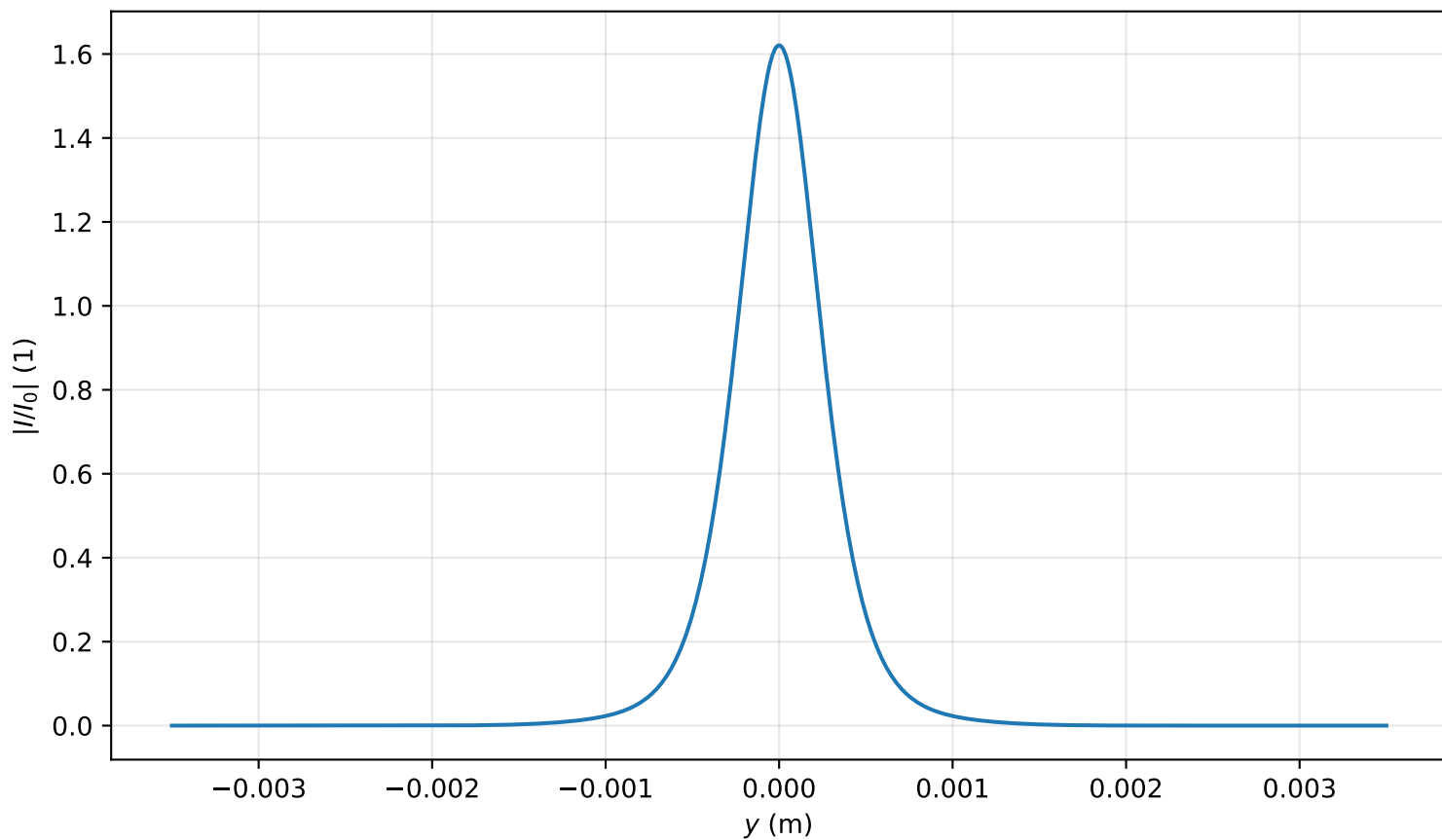
Intensity profile I(x=0, y, z=1.831)/I_0 , P_{in}=0.9P_{cr} , artificial time
